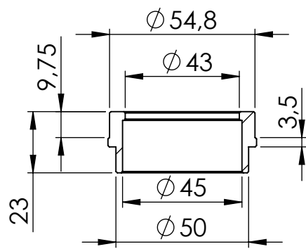
bushing cod.206424R
