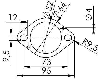
Flange sp.5mm cod.206423R
