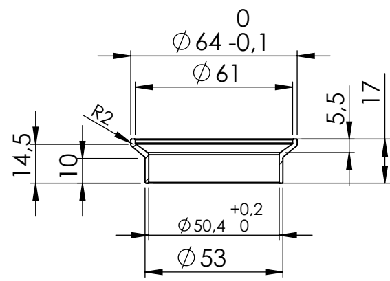
welded bushing
